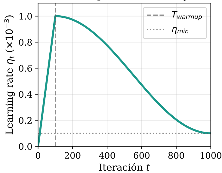
Warmup + Cosine decay
